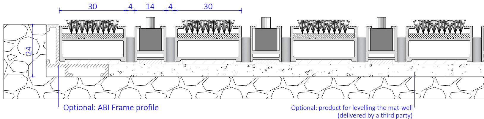
Vertical cross section mat
