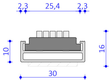
Detail with inlay brushes
