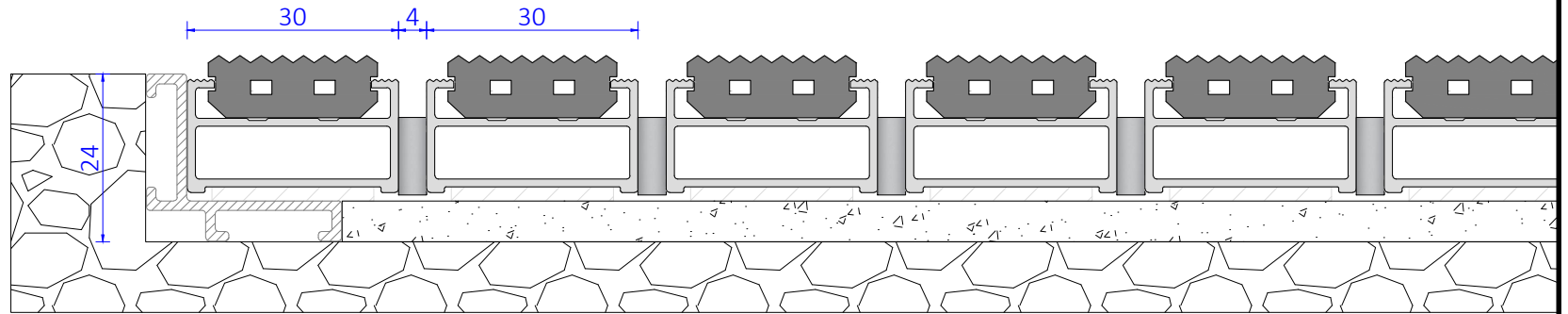
Vertical cross section mat
