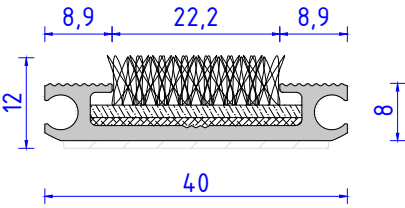
Detail with inlay needlepunch
