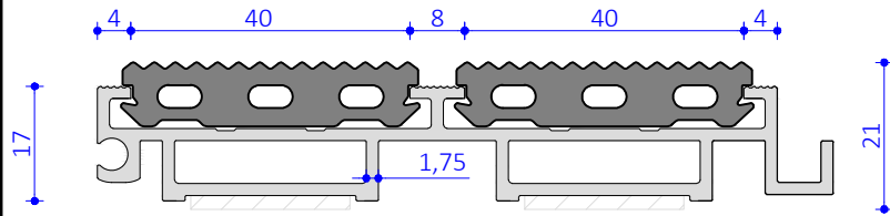
Detail with inlay rubber
